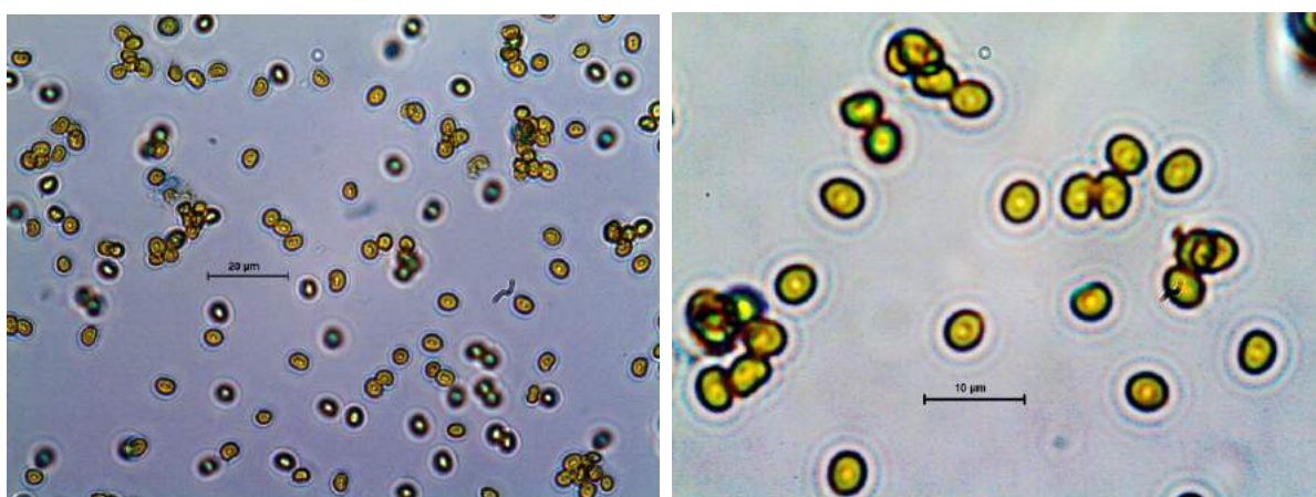
Figs. 7-8. Laetiporus sulphureus , basidiospores
