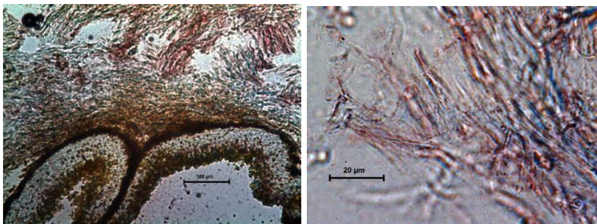
Figs. 5-6. Laetiporus sulphureus , 5 cross section of pore layer, 6 hyphal system,
